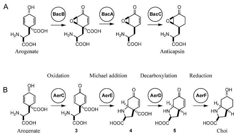
Figure 5. Proposed Biosynthetic Pathways of the Anticapsin Moiety of Bacilysin and the Choi Moiety of Aeruginosin
